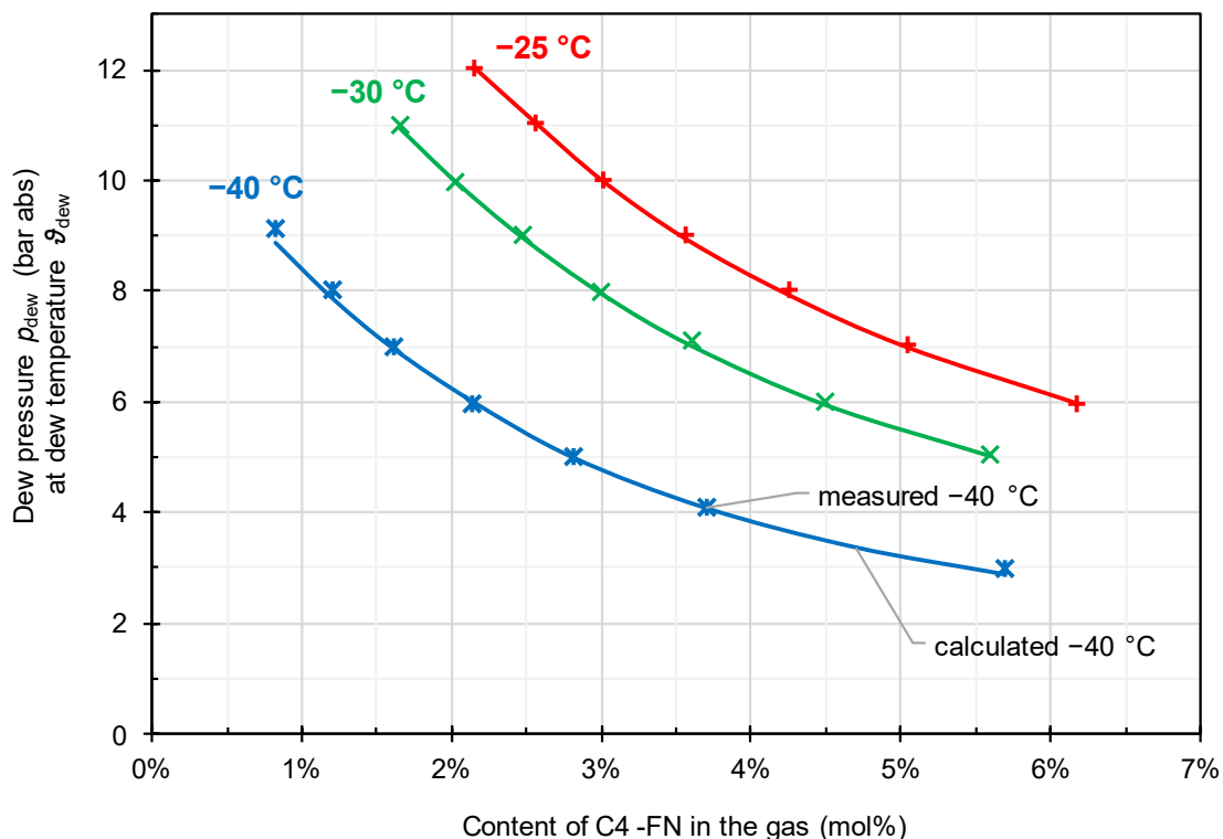
Figure 16: Measured vs. calculated (Eq. (3)) dew curves of C4-FN at -25 °C, -30 °C, and -40 °C, with a O 2 content in the gas phase of 10 % and the rest being CO 2 .
