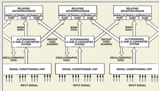
AEP digital substation architecture concept, circa 1980.
