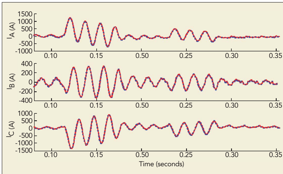
An event on Sept. 30, 2008, recorded on the Hyatt line with hardwired relay (blue) and measured by HardFiber bricks (red).
