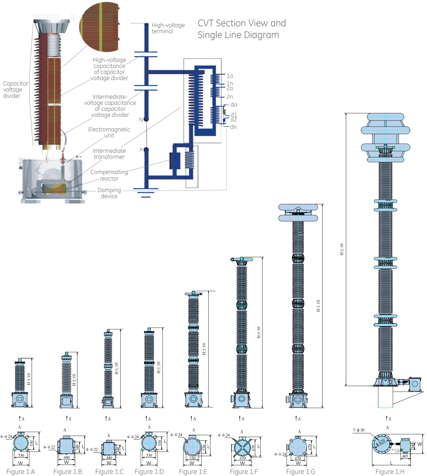
CVT Configuration and Dimensional Drawings
